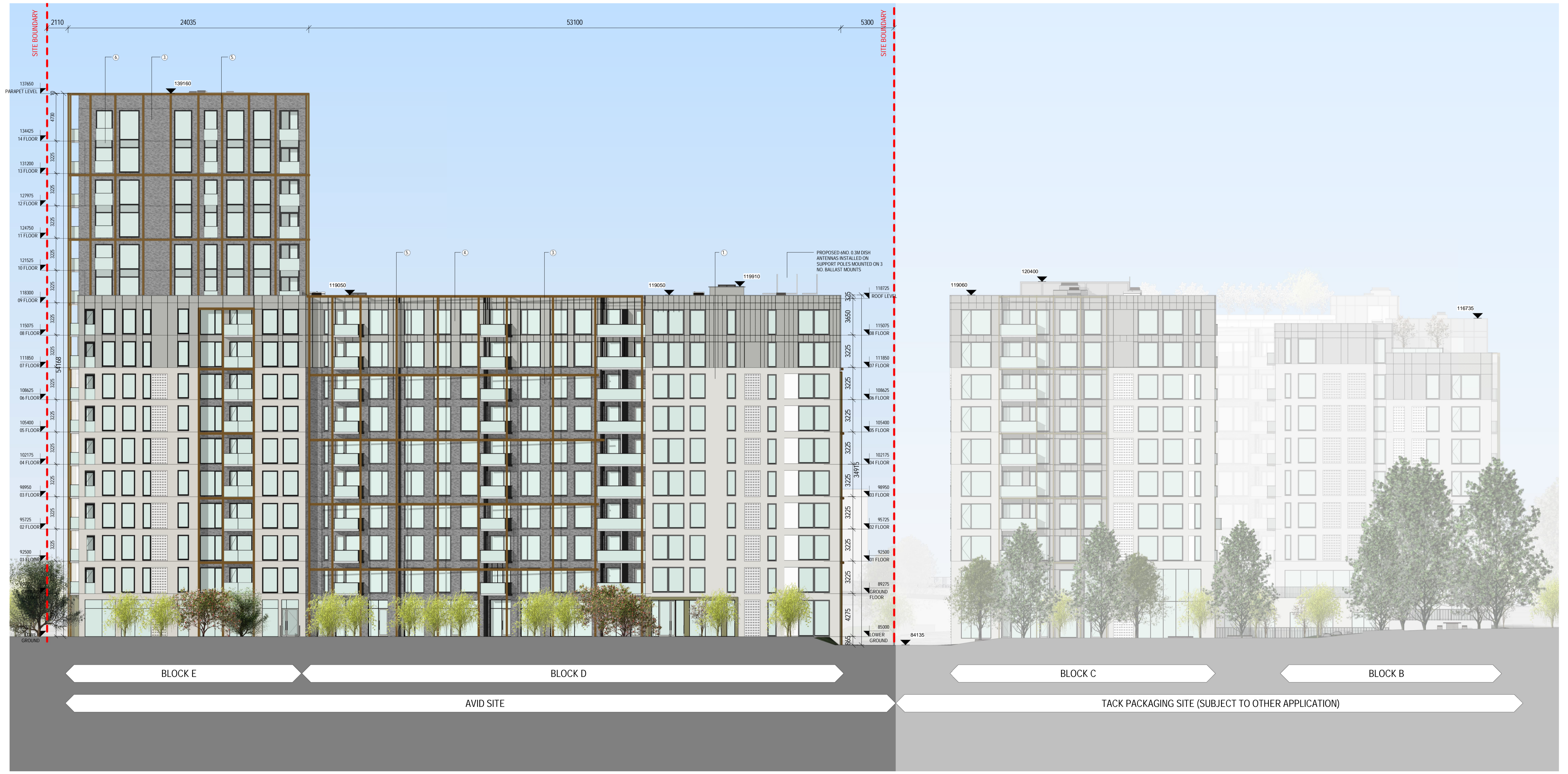
1 PROPOSED NORTH EAST ELEVATION - AVID SITE 1 : 200
